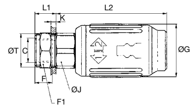
9417U Bulkhead Body NPT – 1/4 I.D.
