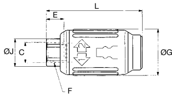
9415U Female Straight Body NPT – 1/4 I.D.
