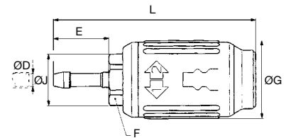
9421U Barbed Connector Body – 1/4 I.D.
