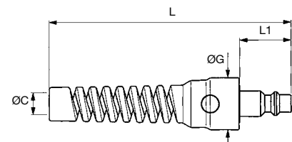
9080U Body + Spring Guard – 1/4 I.D.
