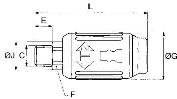
9405U Male Straight Body NPT – 1/4 I.D.
