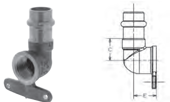
PC707-3-5-A Hi-Ear Elbow P x F – Cast *Lead Free
