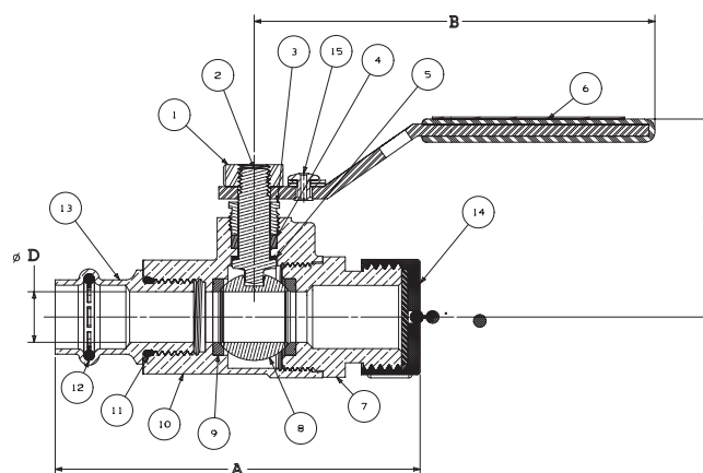
PC-585-66-LF-HC P x Hose
