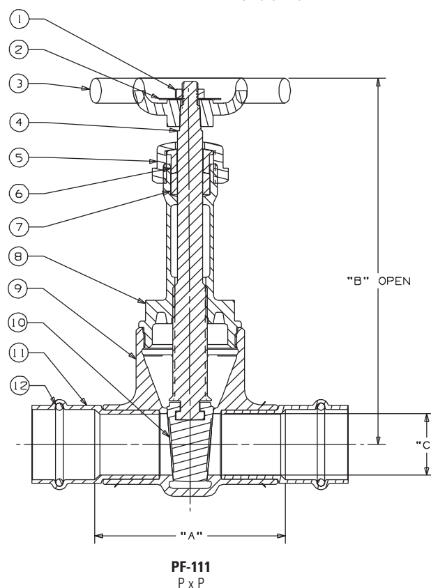
PF-111 Press x Press Female End
