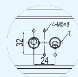
AIR CONNECTION
