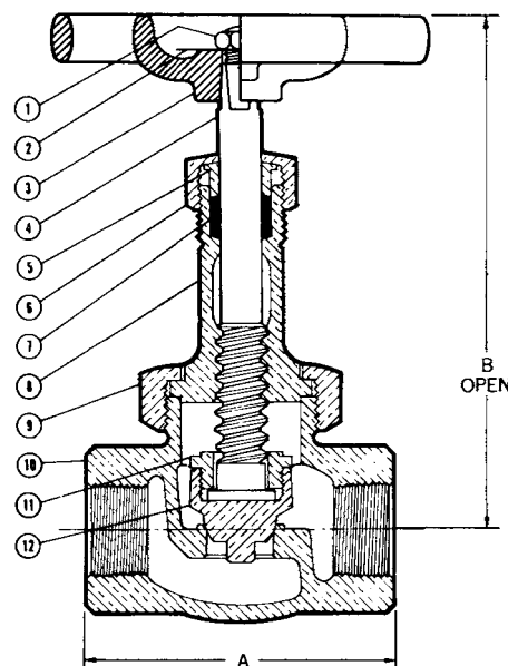
T-275-B NPT x NPT Semi-Plug
