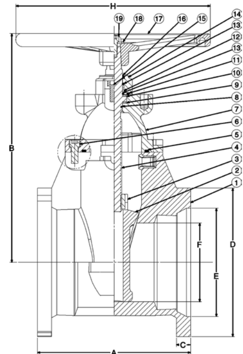
MJ-619-RW MJ x MJ
