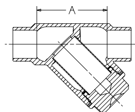
S-221/222-B Solder
