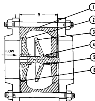
W-910-B/W-960-B Wafer
