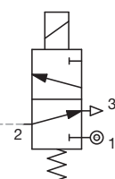
PILOT VALVE
