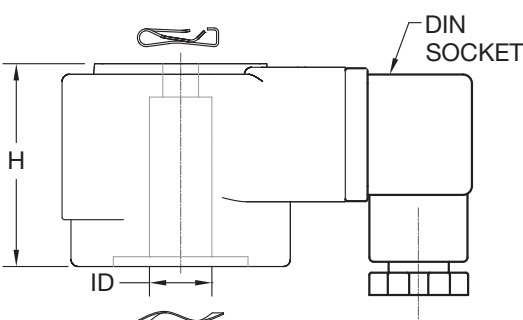
BR COIL
