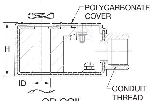
QD COIL
