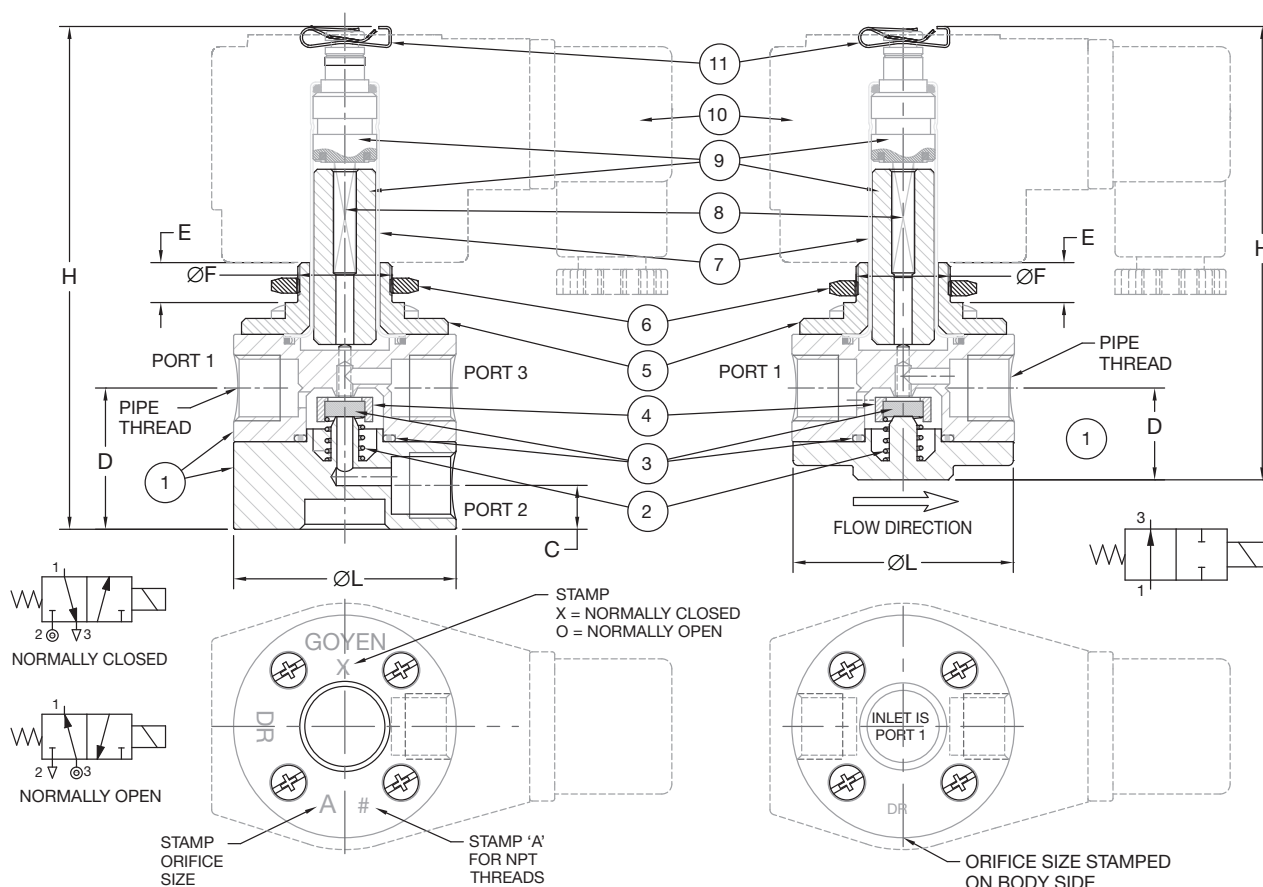
B6M3 CONSTRUCTION
