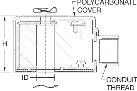
BD COIL
