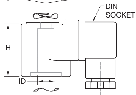
QR COIL
