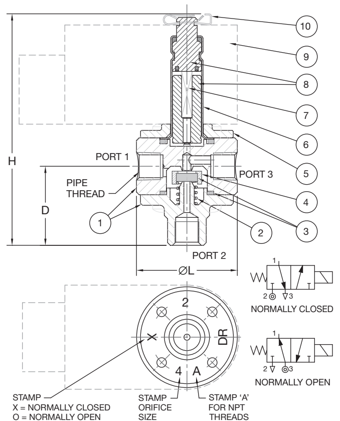
Q3M3T CONSTRUCTION
