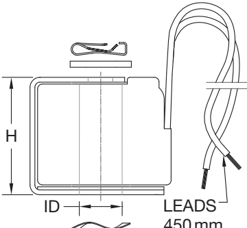
BF COIL
