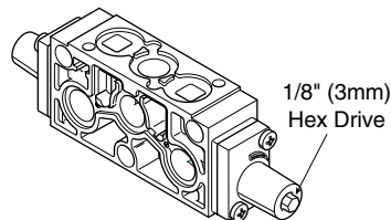
4-Way Manifold with Flow Control
