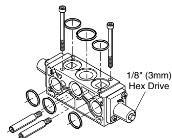
4-Way w/ Flow Control
