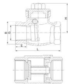
内螺纹止回阀 Female Check Valve
