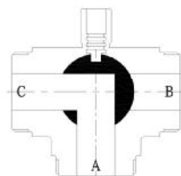
L型球芯 L Port
